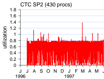
Figure 6: Effect of assuming the wrong number of processors.
